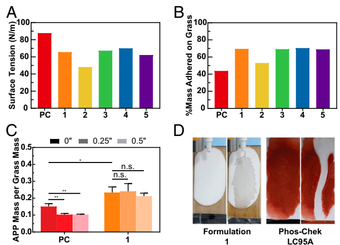
Fig. 2. Vegetation adherence and retention following spray application. (A) Surface tension values for each formulation. (B) Grass was treated by spray application of retardant formulations using a backpack sprayer and the mass adhered on the grass was measured. (C) The treated grass was blended and the phosphorus content was measured using ICP-OES. The mass of APP adhered per mass of grass before and following weathering with simulated rain events was calculated and plotted (mean \pm SD; n = 3 ; 1-way analysis of variance within treatment groups **P < 0.01 , n.s. = not significant; unpaired t test for PC (0 inch) vs. 1 (0 inch) *P \leq 0.05 ). (D) Stability of a dried film of 1 following simulated weathering by dropping water was visibly improved compared to a dried film of PC.
